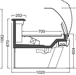
NAVI102-Y-D BLOK AYAK NAVI102-Y-D WITH LEGS
