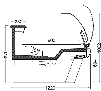
NAVI122-Y-D BLOK AYAK NAVI122-Y-D WITH LEGS
