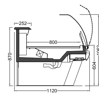
NAVI112-Y-D BLOK AYAK NAVI112-Y-D WITH LEGS
