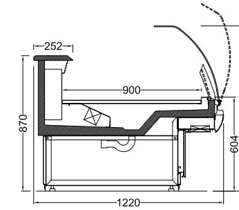
NAVI122-Y-D BAZALI NAVI122-Y-D COVERED BASE
