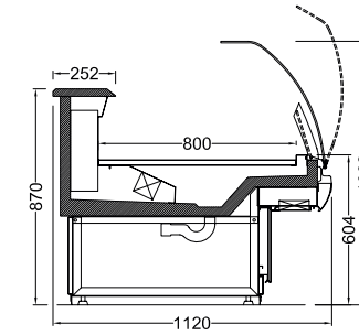
NAVI112-Y-D BAZALI NAVI112-Y-D COVERED BASE
