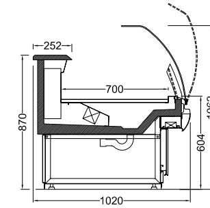
NAVI102-Y-D BAZALI NAVI102-Y-D COVERED BASE
