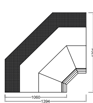
NAVI102-Y-Y/D
