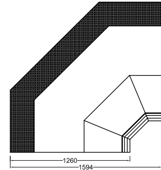
NAVI122-Y-Y/D
