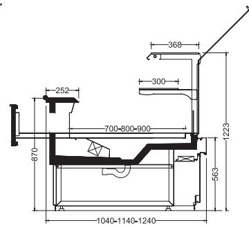
NAVI FLAT-4 PASTA (ÇEKMECELİ) BAZALI NAVI FLAT-4 PASTRY (ON DRAWER) SOLID BASE
