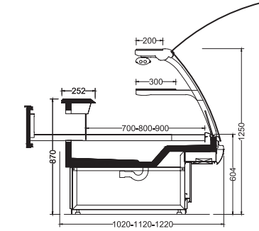
NAVI-YK PASTA (ÇEKMECELİ) BAZALI NAVI-YK PASTRY (ON DRAWER) SOLID BASE
